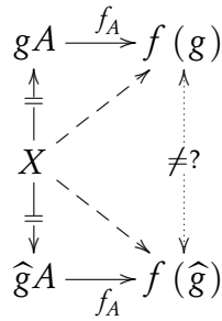
Figure 4.1. Mappings whose domains are quotient groups might not be functions: how do we know that f(g) = f(\widehat{g}) ? If not, then f_A(X) could have two different values.
