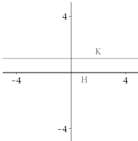
Figure 3.1. H and K from Example 3.8
